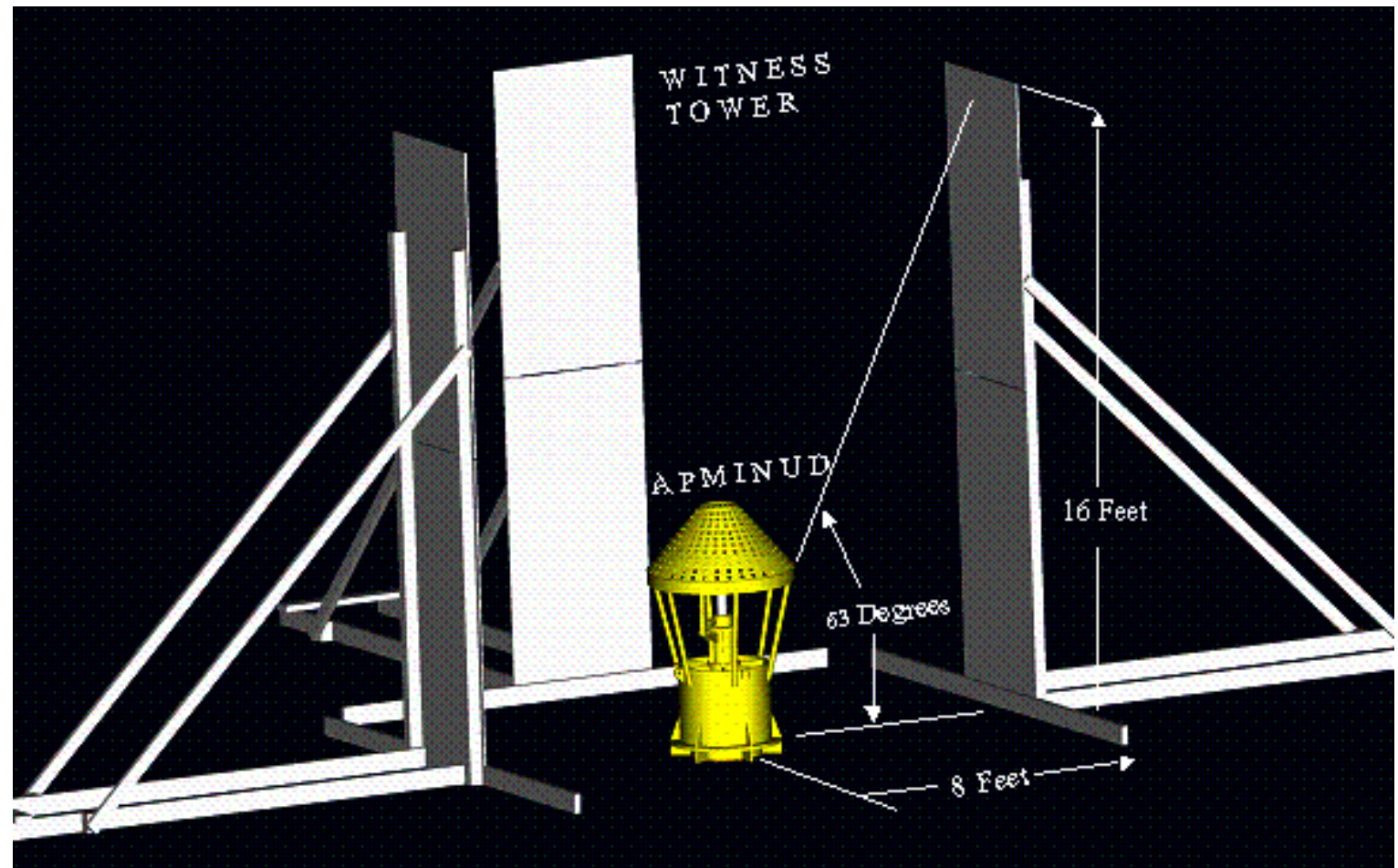
FIGURE 4. Explosive Test Set Up and Witness Tower Placement
